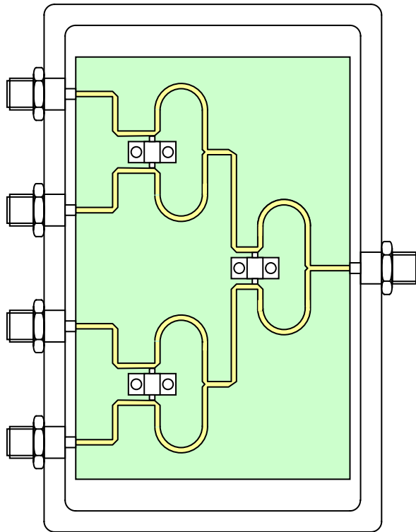
Narrow band four port combiner/splitter, Wilkinson circuit.
