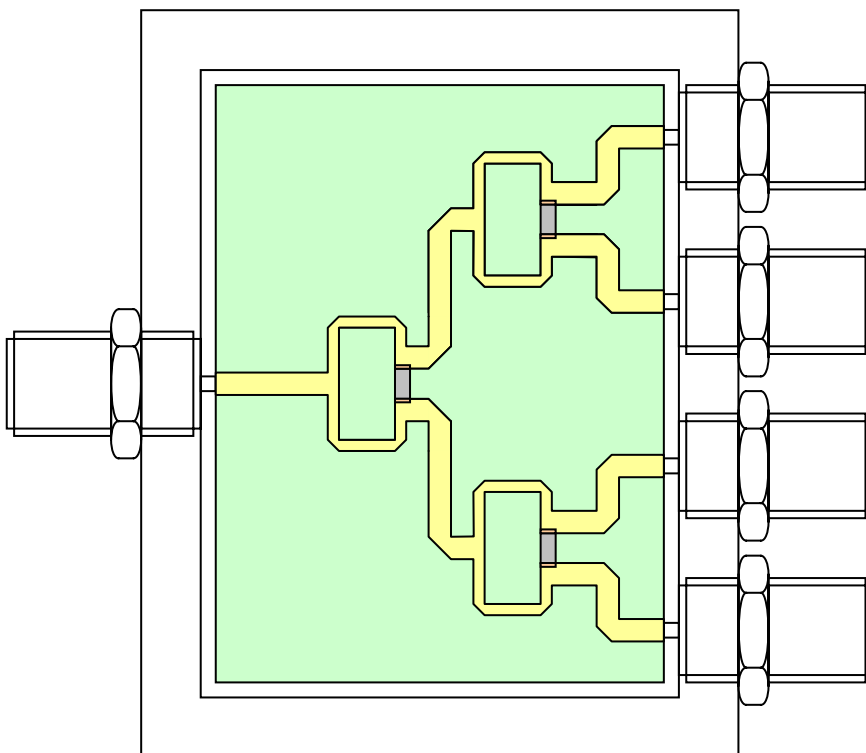
Narrow band four port splitter, Wilkinson circuit.
